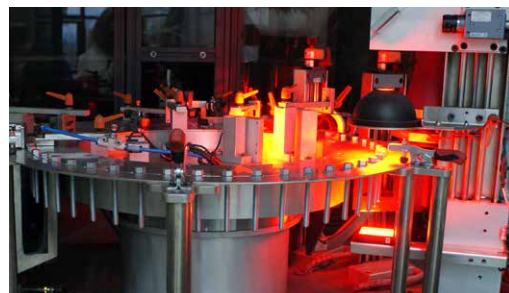
Pomiar zarysu i kontrola optyczna Measurement of outline and optical inspection
